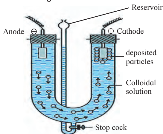
Fig. 11.10 : Electrophoresis
