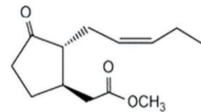
Methyl jasmonate
